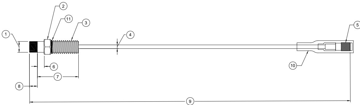
FIGURE 5: MX2030 8mm Reverse-Mount Probe (AA=05 and 06)
