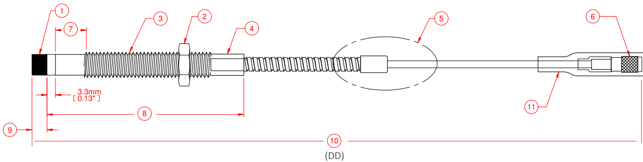
FIGURE 4: MX2030 8mm Forward-Mount Probe (AA=01 through 04)
