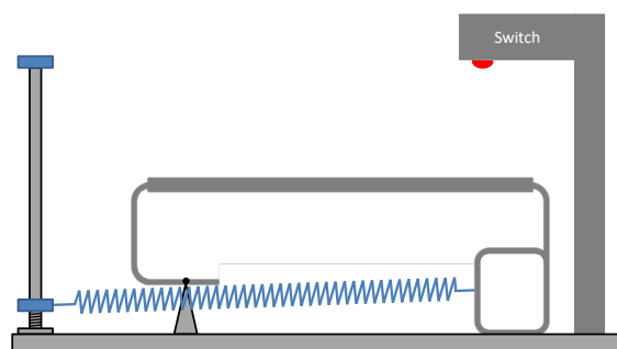
Figure A: 5550 mechanical switch trip mechanism in untripped position. Micro-switch (red) is not actuated.
