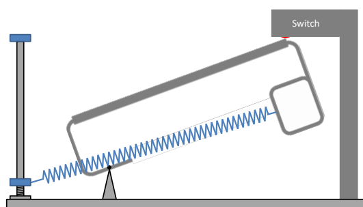
Figure B: 5550 mechanical switch trip mechanism in tripped position. Micro-switch (red) is actuated.
