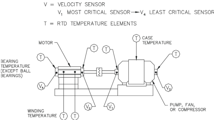
Figure 1: Horizontal mounting for casing vibration measurements.
