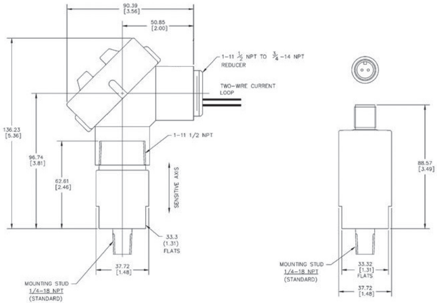
Figure 10: Outline dimensions of the ST5484E-XXX-XX4-XX (MIL-Style Connector). Dimensions in mm [inches].
