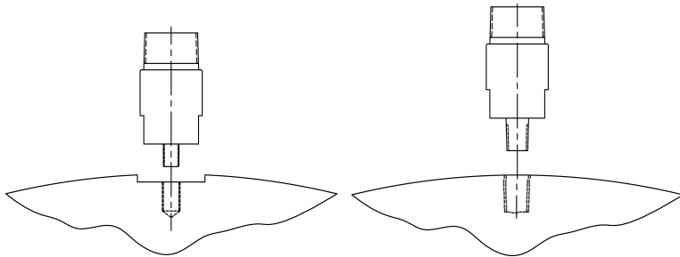
Machine thread style requires prepared surface (spot facing) for bottom contact
