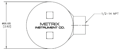
Figure 8: Outline dimensions of the ST5484E (with the optional 8200 Stainless Steel Conduit Elbow installed).
