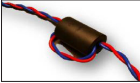
Figure 4: Leads may also be looped through the ferrite core (Metrix PN 100463) to attenuate different frequencies. The optimal number of loops will vary by application and the interfering frequency(ies). The wrapped ferrite core should be placed in the 8200 Conduit Elbow or equivalent.
