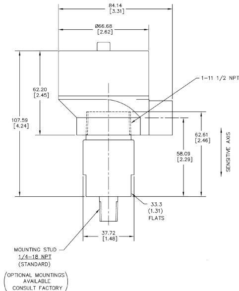
Figure 8: Outline dimensions of the ST5484E (with the optional 8200 Stainless Steel Conduit Elbow installed).
