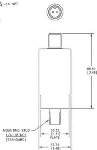
Figure 9: Outline dimensions of the ST5484E-XXX-XX4-XX (MIL-Style Connector). Dimensions in mm [inches].
