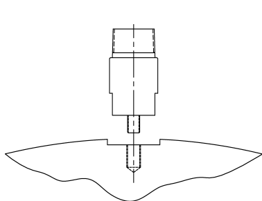
Machine thread style requires prepared surface (spot facing) for bottom contact
