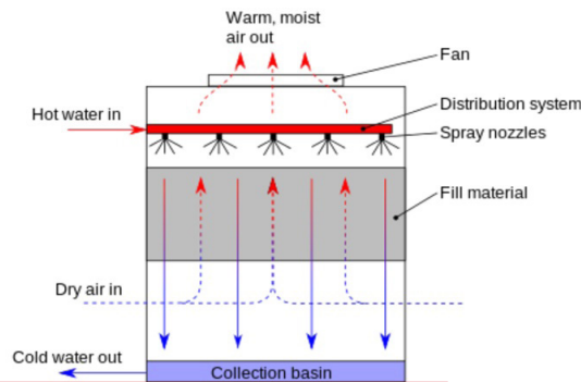
Counterflow Cooling Tower
