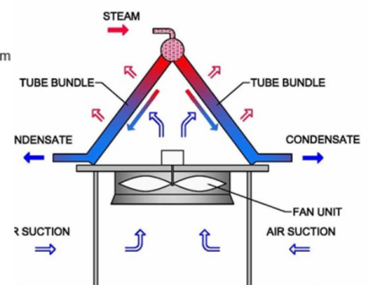
Dry Cooling Tower
